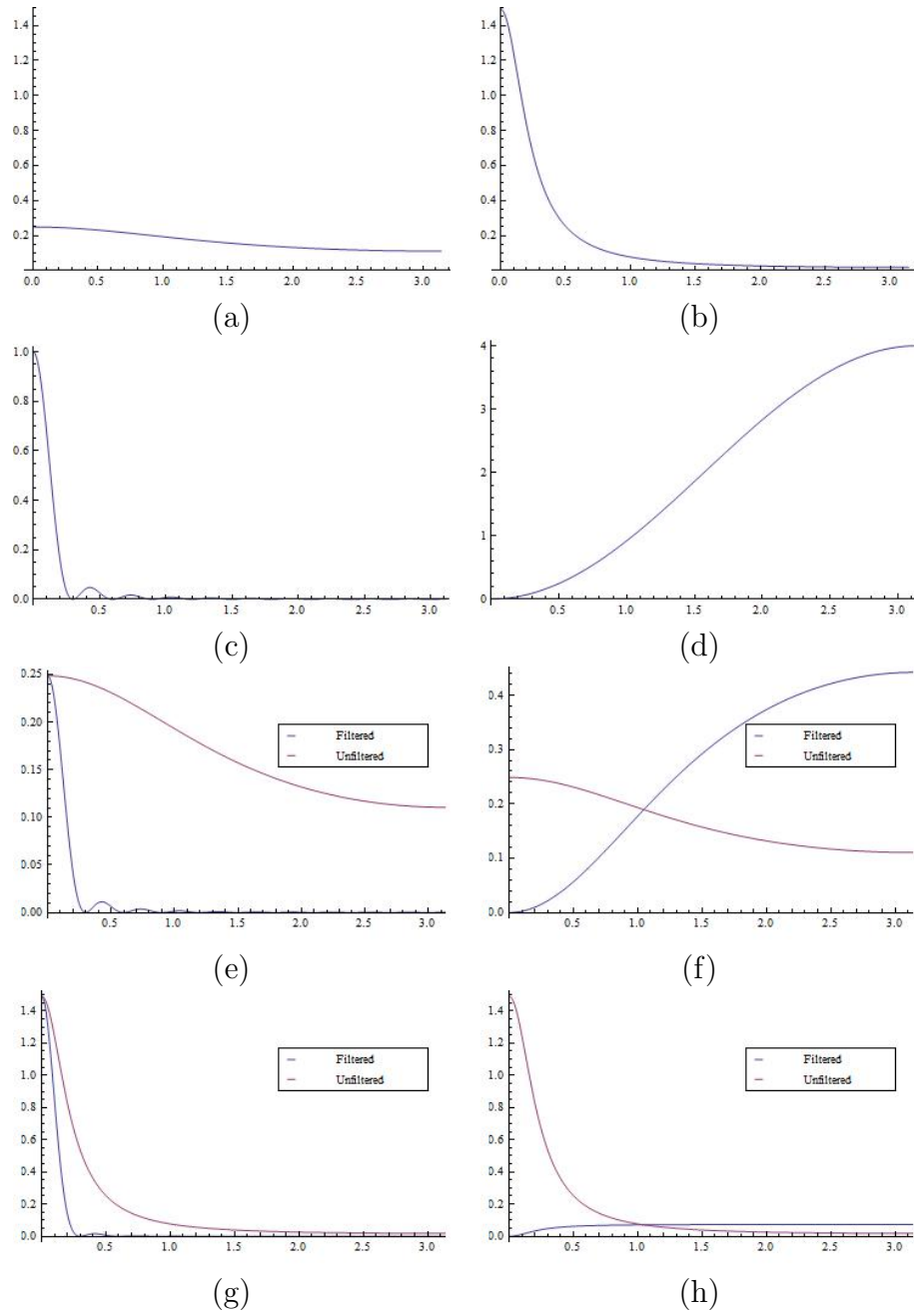
Figure A.1: Two processes, two filters - an example: (a) Spectrum of noisy AR(1), (b) Spectrum of smooth AR1, (c) PTF of MA filter, (d) PTF of difference filter, (e) MA filtered and unfiltered noisy AR1, (f) Difference filtered and unfiltered noisy AR1, (g) MA filtered and unfiltered smooth AR1, (h) Difference filtered and unfiltered smooth AR1
