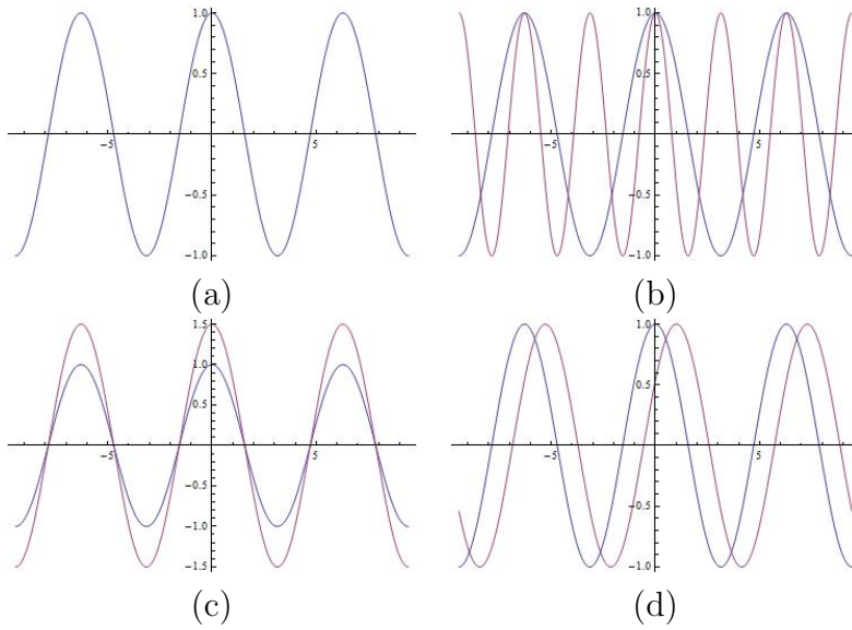
Figure 1: Cycles plotted for different (\omega, \rho, \theta) : (a) (1, 1, 0) , (b) (2, 1, 0) , (c) (1, 1.5, 0) , (d) (1, 1, 1)
