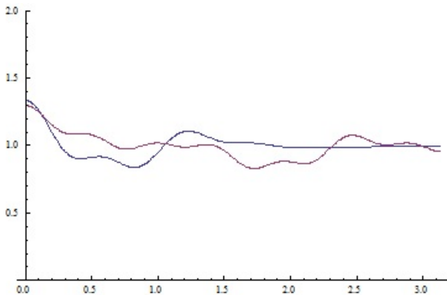
Figure 4: Power transfer functions implied by the bank's filter choice - Blue: Regulator band [0.20, 1.05] , Red: Regulator band
