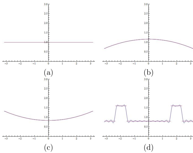
Figure A.3: A collection of illustrative penalty functions (and finite approximations): (a) Equal across \omega , (b) Greater at low \omega , (c) Greater at high \omega , (d) Heavy in a particular band
