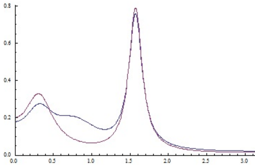
Figure 9: Approximation to a particular spectral density obtained by a combination of stochastic cycles - red: target density, blue: approximation
