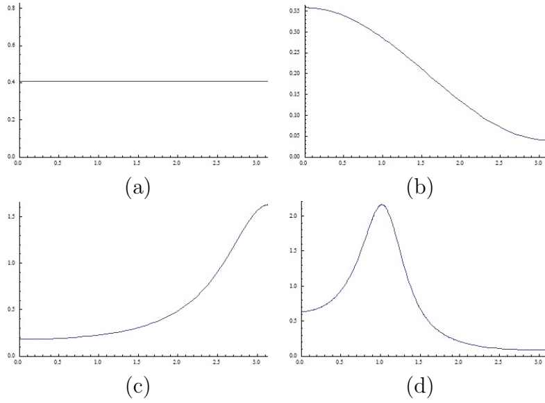
Figure 2: Spectral densities for different processes: (a) White Noise, (b) MA(1) \theta = 0.5 , (c) AR(1) \phi = -0.5 , (d) AR(2) \phi_1 = 0.7, \phi_2 = -0.5
