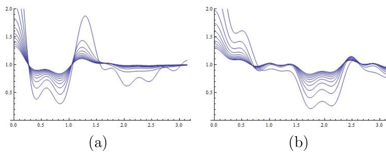
Figure 5: Power transfer functions implied by the bank's filter choice - under different penalization weights: (a) Regulator band [0.20, 1.05] (b) Regulator band [1.57, 2.34]
