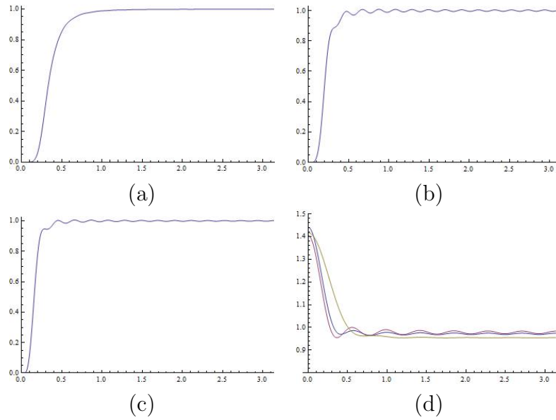
Figure 6: Hodrick-Prescott (approx.) filters and the associated power transfer function responses of the bank: (a) \lambda = 200 , (b) \lambda = 1600 , (c) \lambda = 4600 (d) PTF
