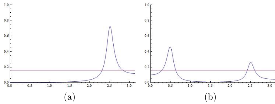
Figure 10: Spectral densities of portfolios compared to uncontrolled spectral density - (a) No penalty, (b) Constant penalty
