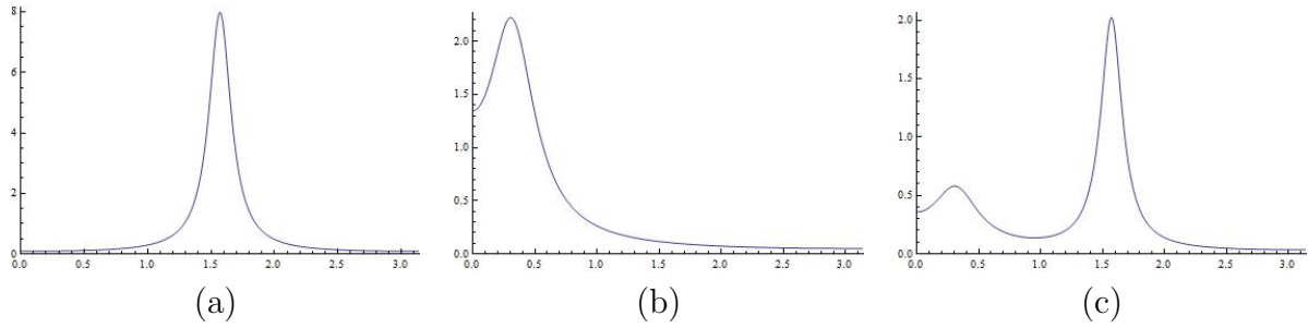
Figure 8: Two stochastic cycles and their combination: (a) \lambda = \frac{\pi}{2} , \rho = 0.9 , (b) \lambda = \frac{\pi}{10} , \rho = 0.8 , (c) (0.5, 0.5) weights
